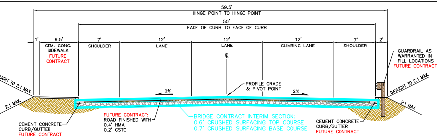
EASTMONT EXTENSION ROADWAY SECTION NO SCALE
