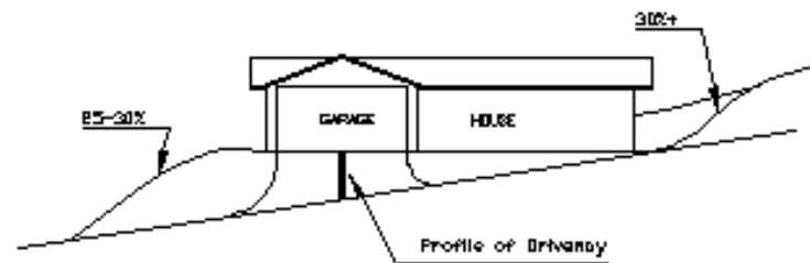
DRIVEWAY ELEVATION
