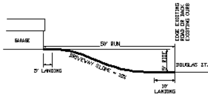
DRIVEWAY PROFILE
